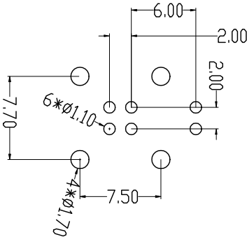
PCB Layout Reference
